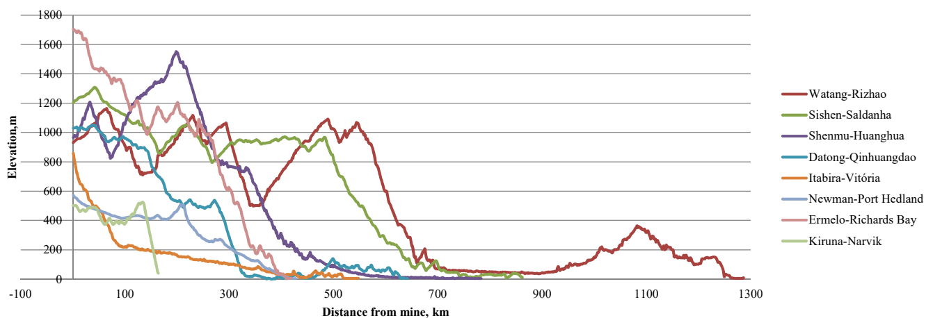
Vertical alignments of the eight heavy haul cases
